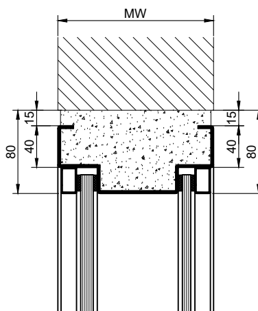
Blockzarge
